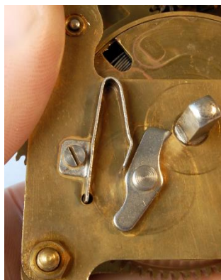
Figure 74 – click spring in situ
