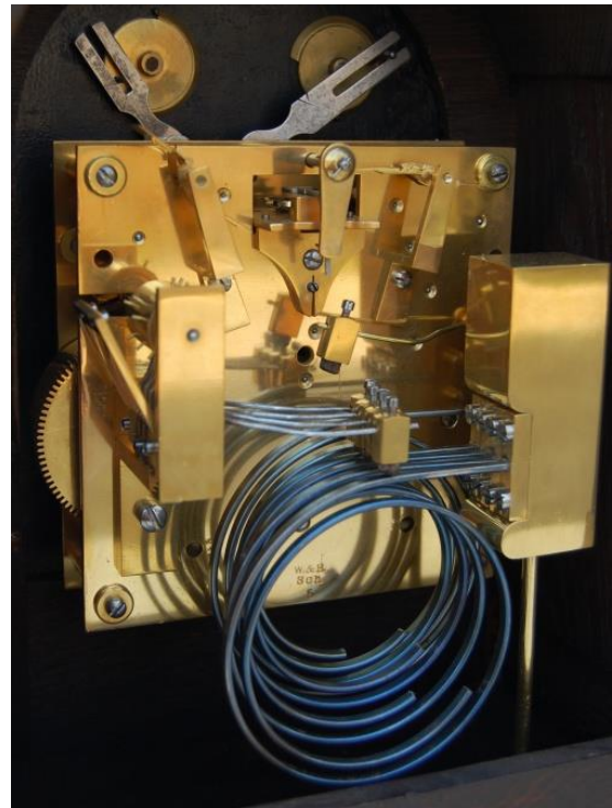
Figure 30 – rear view of a high quality chiming clock
